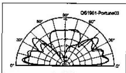
Figure 3 — Vertical radiation plot of the slot-cube antenna (blue) compared with a J-pole antenna (red).
