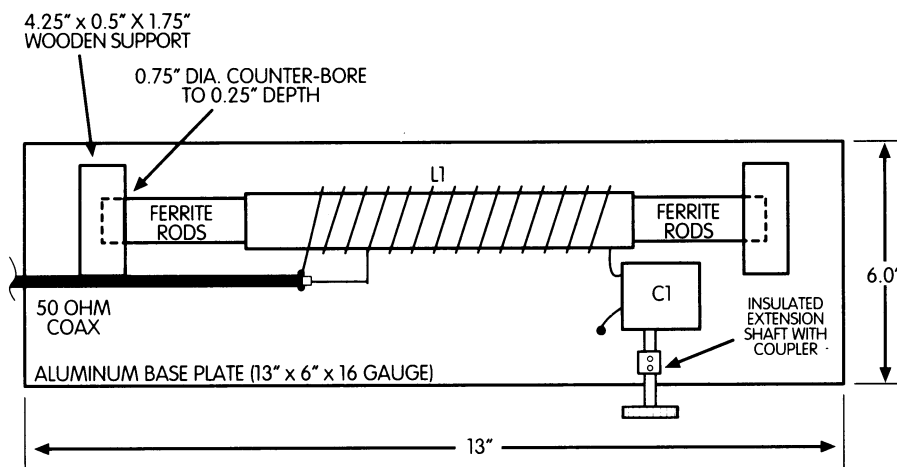
Fig. 7. Assembly, top view.
