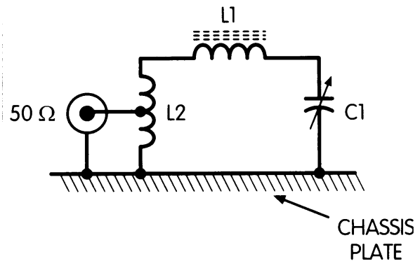
Fig. 3. A successful TX ferrite loop. Much easier to adjust than Fig. 2.
