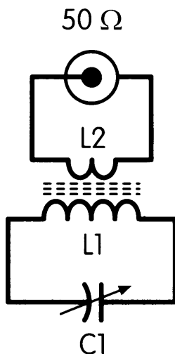
Fig. 1. The conventional ferrite loop. OK "on receive" only.
