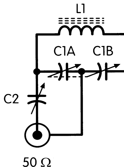
Fig. 2. An earlier TX ferrite loop. Successful, but very difficult to adjust and QSY.
