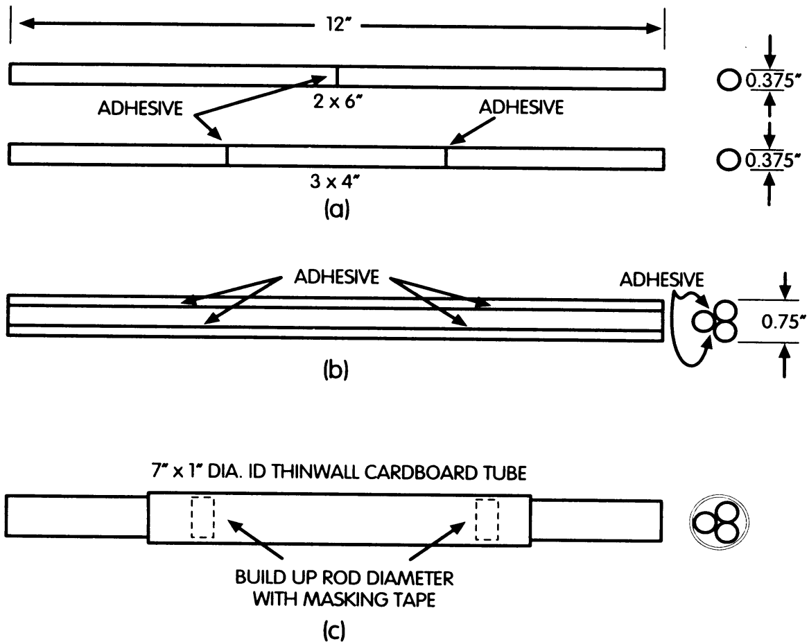
Fig. 5. Assembly of 3/4" ferrite rod and coil former for L1. (A) Fabrication of 12" x 3/8"-diameter rods. (B) Fabrication of 12" x 3/4"-diameter ferrite rod. (C) Assembly of coil L1 former on "B".
