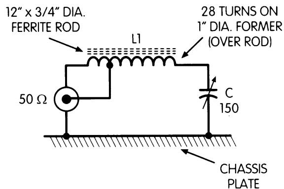
Fig. 4. Schematic of author's 1997 80–160 m ferrite TX loop. L1 = 28 spaced wire turns tapped 2-3/4 turns for Z = 50 ohms. C = 150 pF small, TX-type variable.
