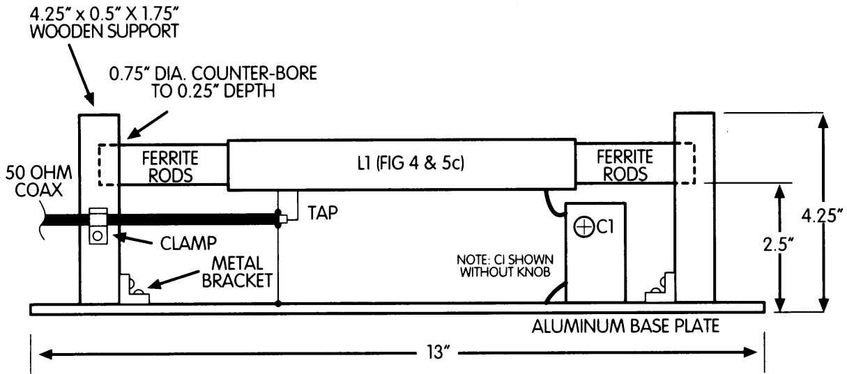
Fig. 6. Assembly, side view.
