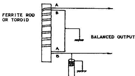
UNBALANCED FEEDER TO A.T.U.
